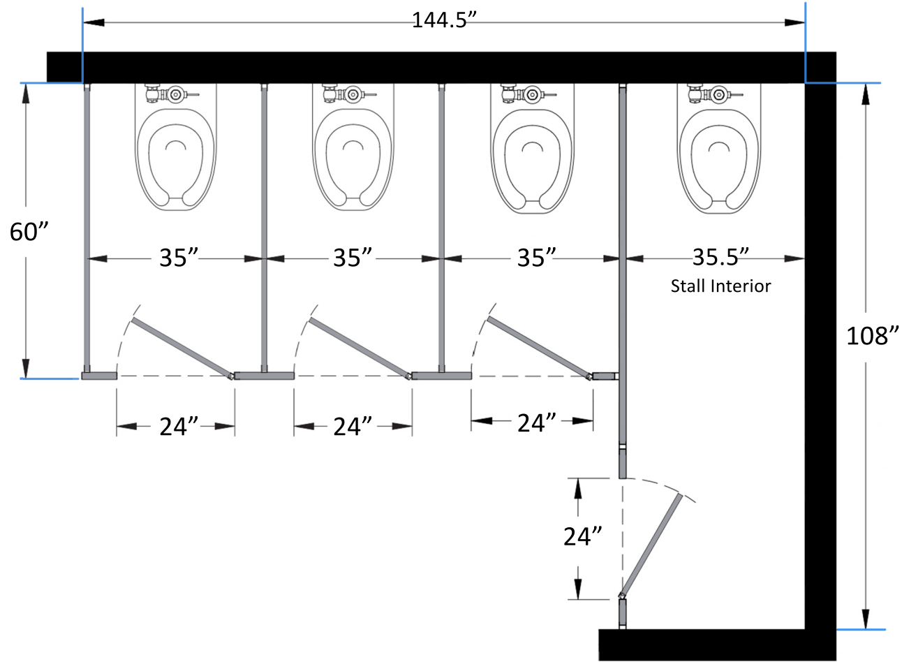
Bathroom Partitions - 4 Stall Alcove Right Hand SKU: ALIC4R Standard Dimensions
